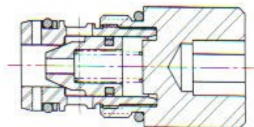
Anti-cavitation Check
