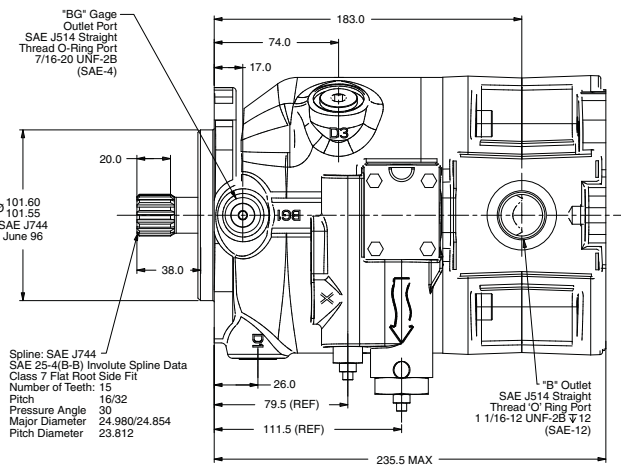
P1/PD 028 Port Sizes
